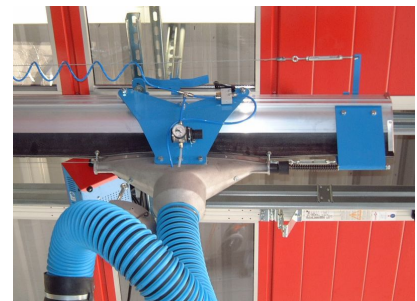
Detail Saugwagen
